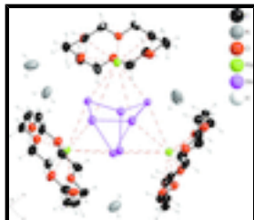
Fig. 1. : Asymmetric unit of the compound [\text{Rb}(\text{18-crown-6})]_3\text{Sb}_7.4\text{NH}_3 . Ellipsoids of all non-hydrogen atoms are given with a probability factor of 70%.
