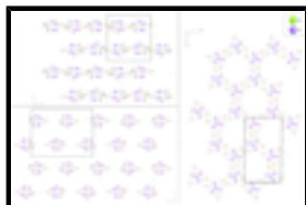
Fig. 2. : Packing of the [\text{Rb}(\text{18-crown-6})]_3\text{Sb}_7 units in each crystallographic direction. Crown ethers and ammonia molecules are omitted. The probability factor of the mapped atoms is 70%.
